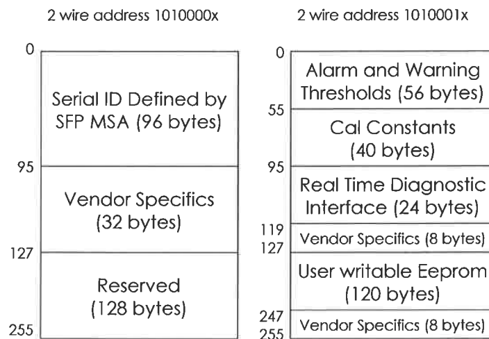
Figure 3. EEPROM of a SFP+
